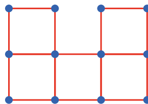
G_2
