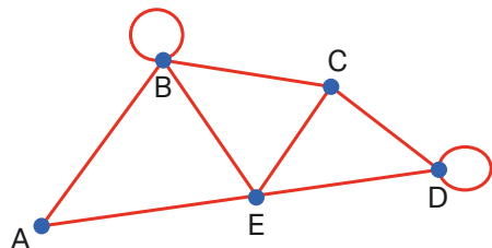
G_1
