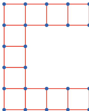
G_4
