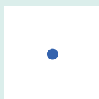
K_1
