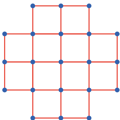
G_5
