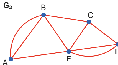
G_2
